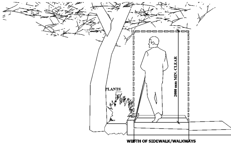
Fig. B.3.7: SIDEWALK/WALKWAY HEADROOM
