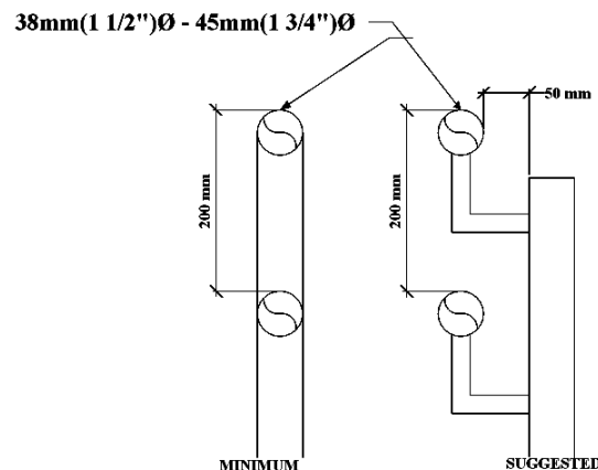
Fig A.3.3 EASY TO GRASP DESIGN
