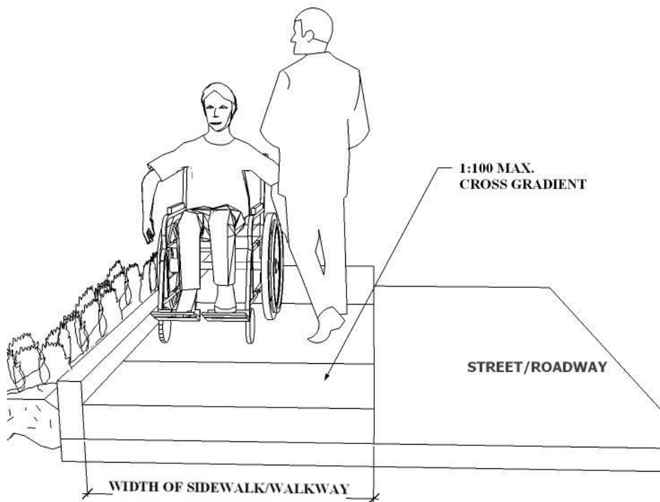
Fig. B.3.1: SIDEWALK / WALKWAYS
