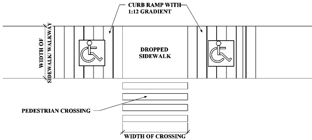
Fig. B.1.2: Plan of DROPPED SIDEWALK
