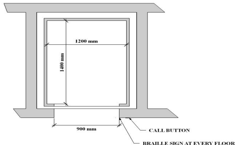
Fig. C.7.2 FLOOR PLAN
