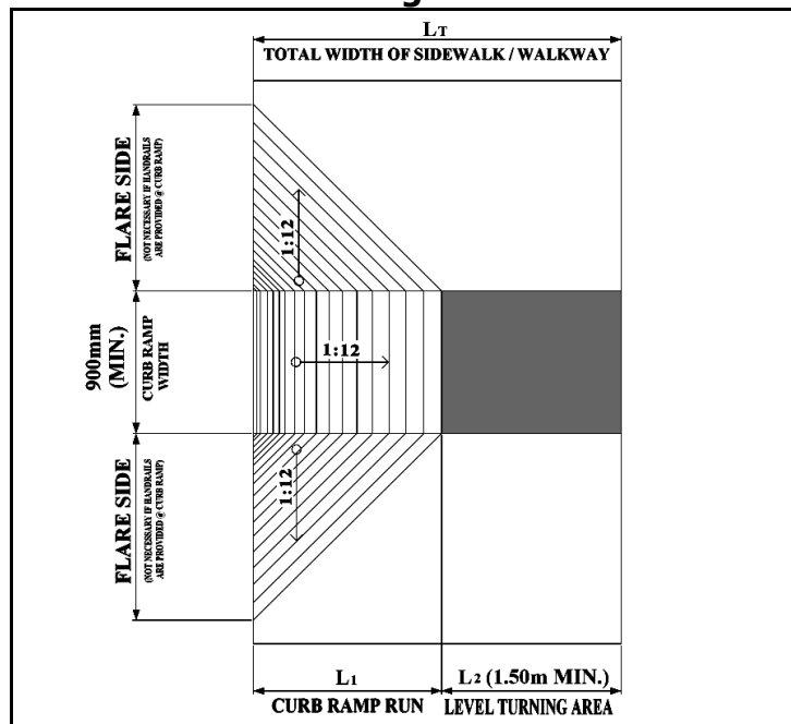
Fig. B.2.3: CURB RAMP
