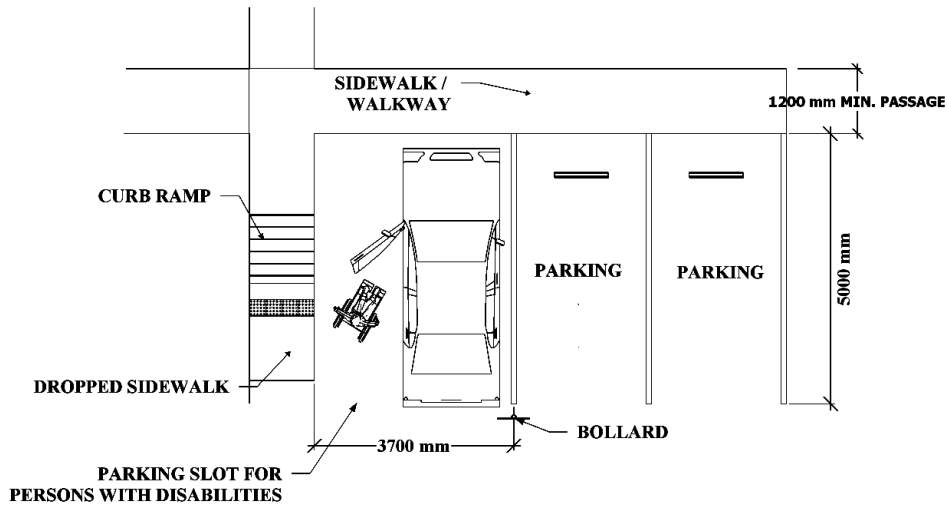
Fig. A.4.1: ACCESSIBLE PARKING SLOT (PLAN)
