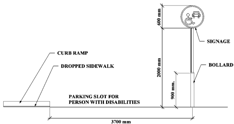
Fig. A.4.3: ACCESSIBLE PARKING SLOT (SHOWING UPRIGHT/POLE MOUNTED SIGNAGE)
