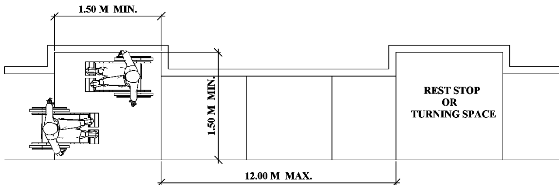
Fig. B.3.3: REST STOP ON BUSY OR LENGTHY SIDEWALK / WALKWAYS
