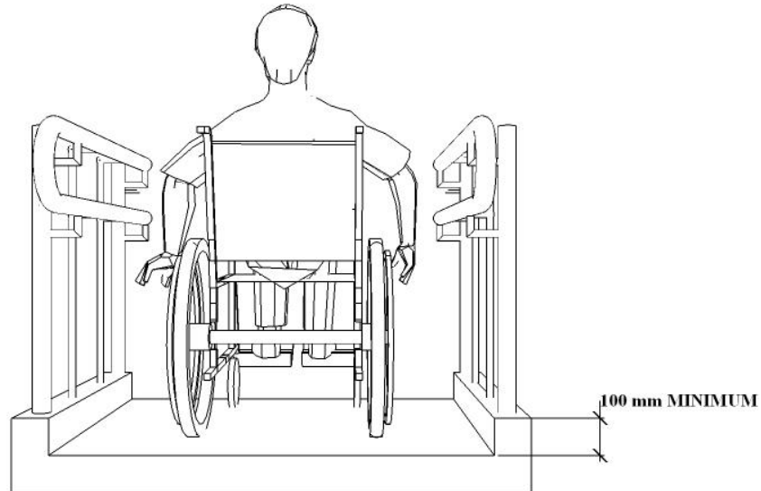
Fig. A.1.5 CURB HEIGHT AT RAMP
