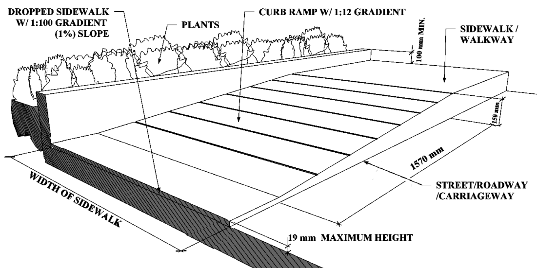
Fig. B.1.4: SECTION OF DROPPED SIDEWALK
