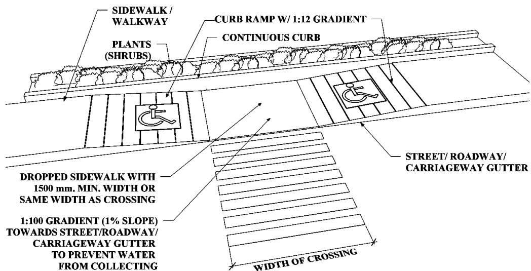
FIG. B.1.1 Perspective of Dropped Sidewalk
