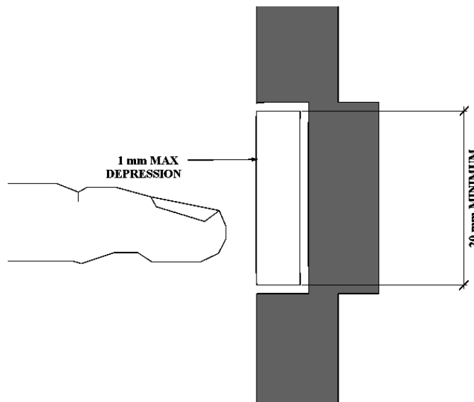
Fig. C.7.4 BUTTON SIZES
