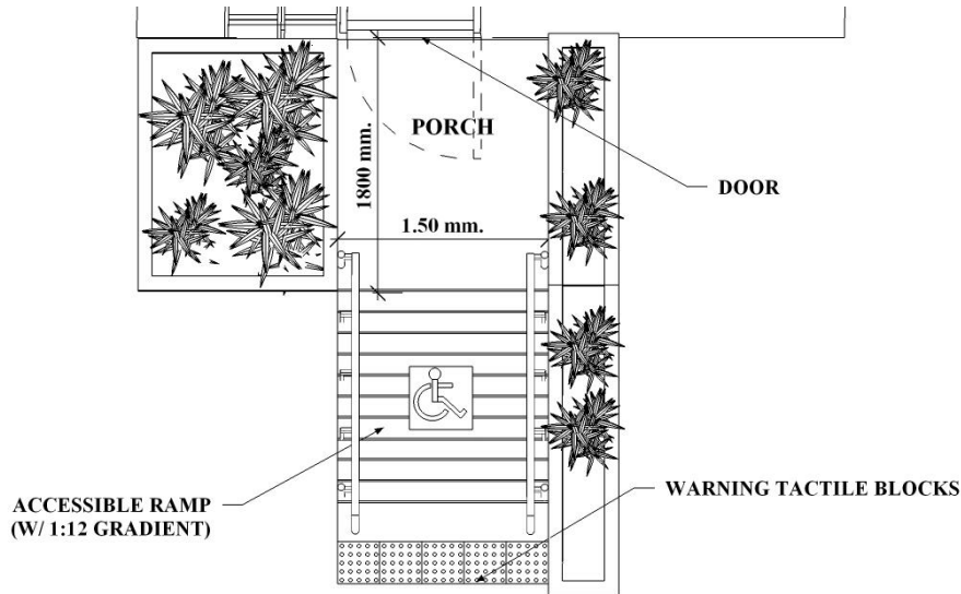
Fig. C.1.2 ENTRANCES WITH VESTIBULES
