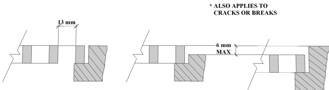
Fig. B.3.2: GRATINGS
