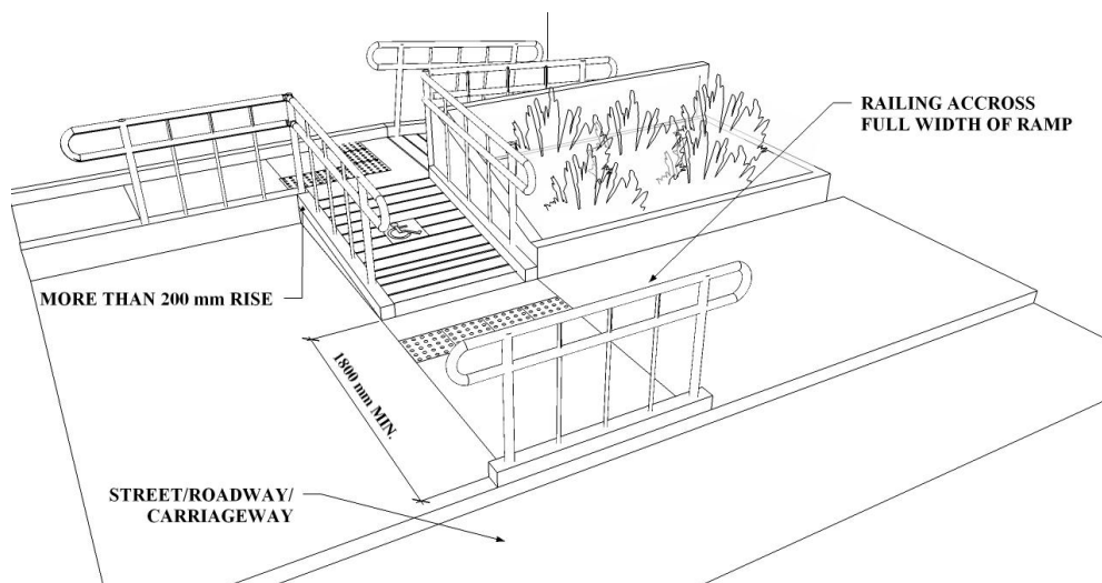
Fig. A.1.6 RAMPS & VEHICULAR TRAFFIC
