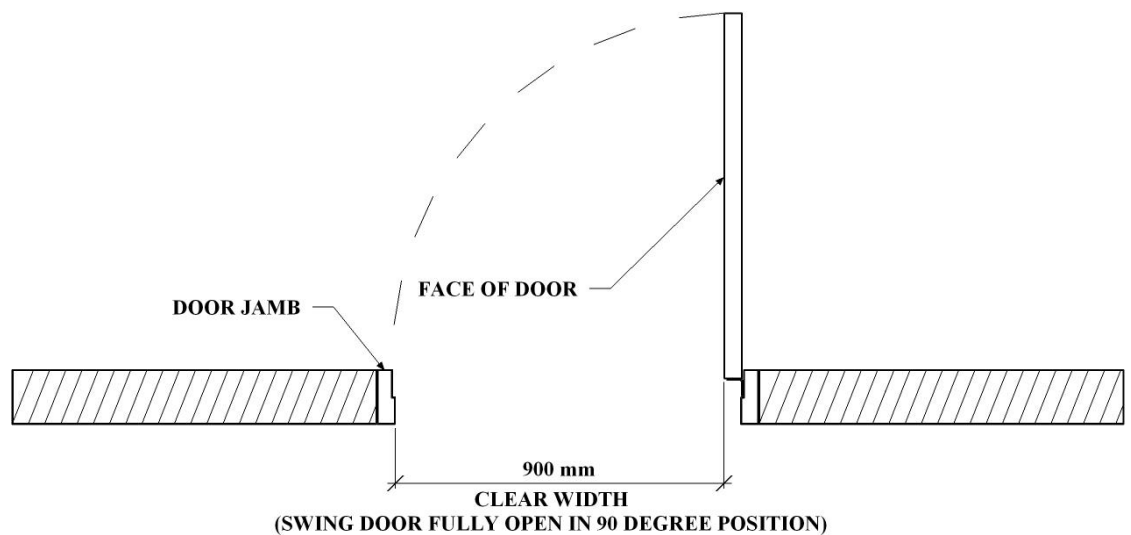
Fig. C.2.2 Plan of SWING DOOR
