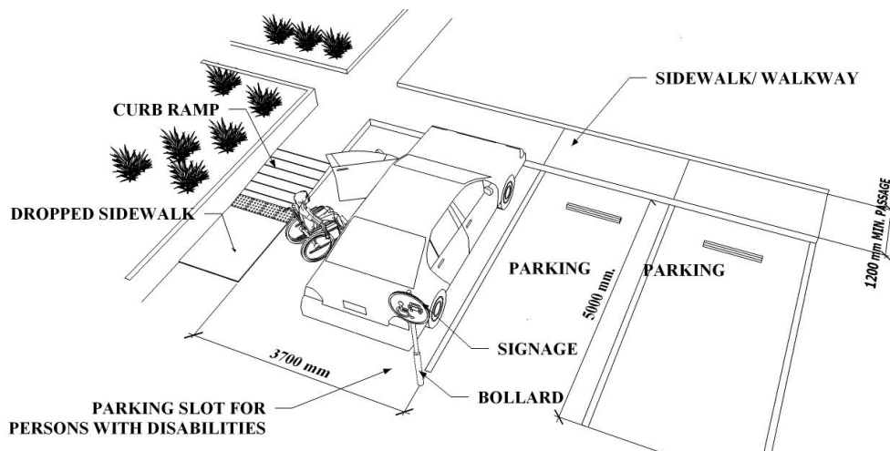
Fig. A.4.2: ACCESSIBLE PARKING SLOT (3D VIEW)
