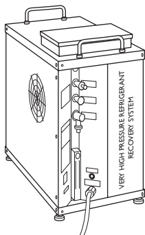
Fig. 7-4 Redi/Controls Refrigerant Mizer Model RS-503/13H Refrigerant Recovery Unit
