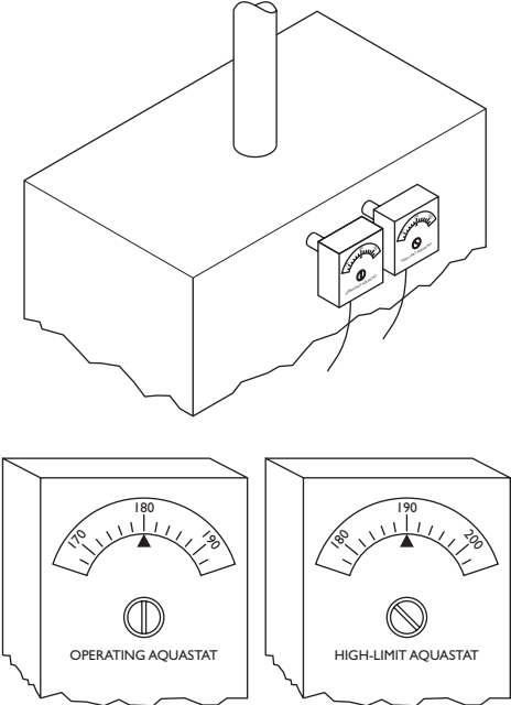
Fig. 6-9 Two aquastats must be used on hot-water boilers
