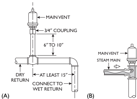
Fig. 5-5 (A) The correct location for an end-of-main vent, (B) The wrong location for an end-of-main vent
