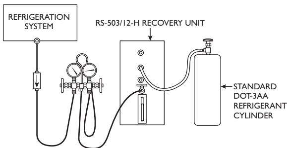
Fig. 7-5 A typical recovery system hookup using the RS-503/13H unit (Courtesy Redi/Controls Inc.)
