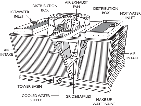
Fig. 7-2 Cutaway view of a cooling tower
