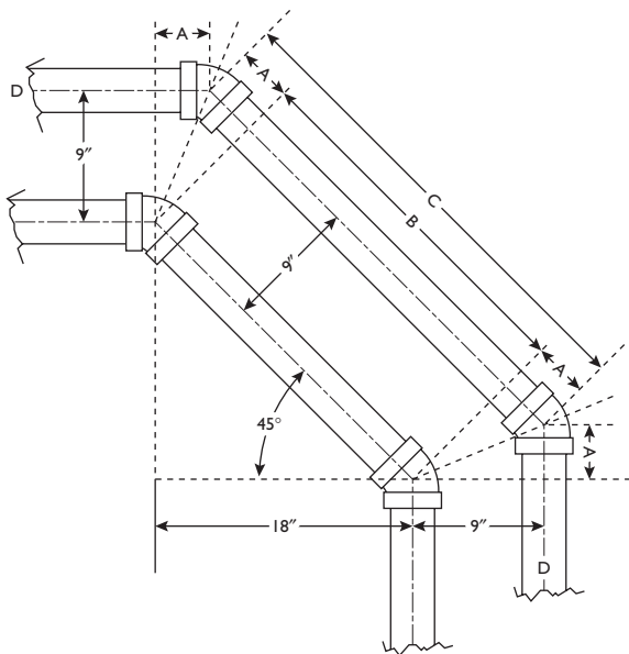
Fig. 2-3 A two-pipe 45° equal-spread offset at a corner
