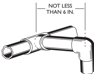
Fig. 12-3 Connection of a drop branch to a horizontal pipe
