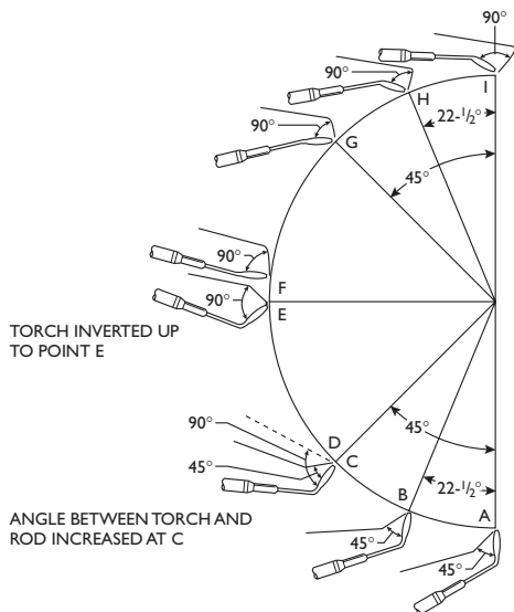
Fig. 3-10 Holding the torch and rod correctly for a position weld
