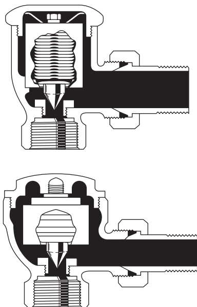
Fig. 5-18 Two types of thermostatic traps
