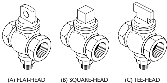
Fig. 6-13 Three types of balancing cocks
