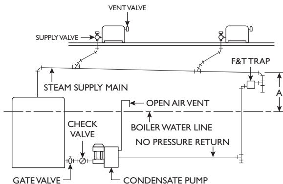
Fig. 5-10 A condensate receiver and pump installed aboveground
