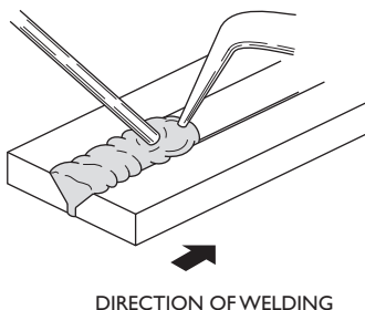
Fig. 3-8 Forehand and backhand welding techniques
